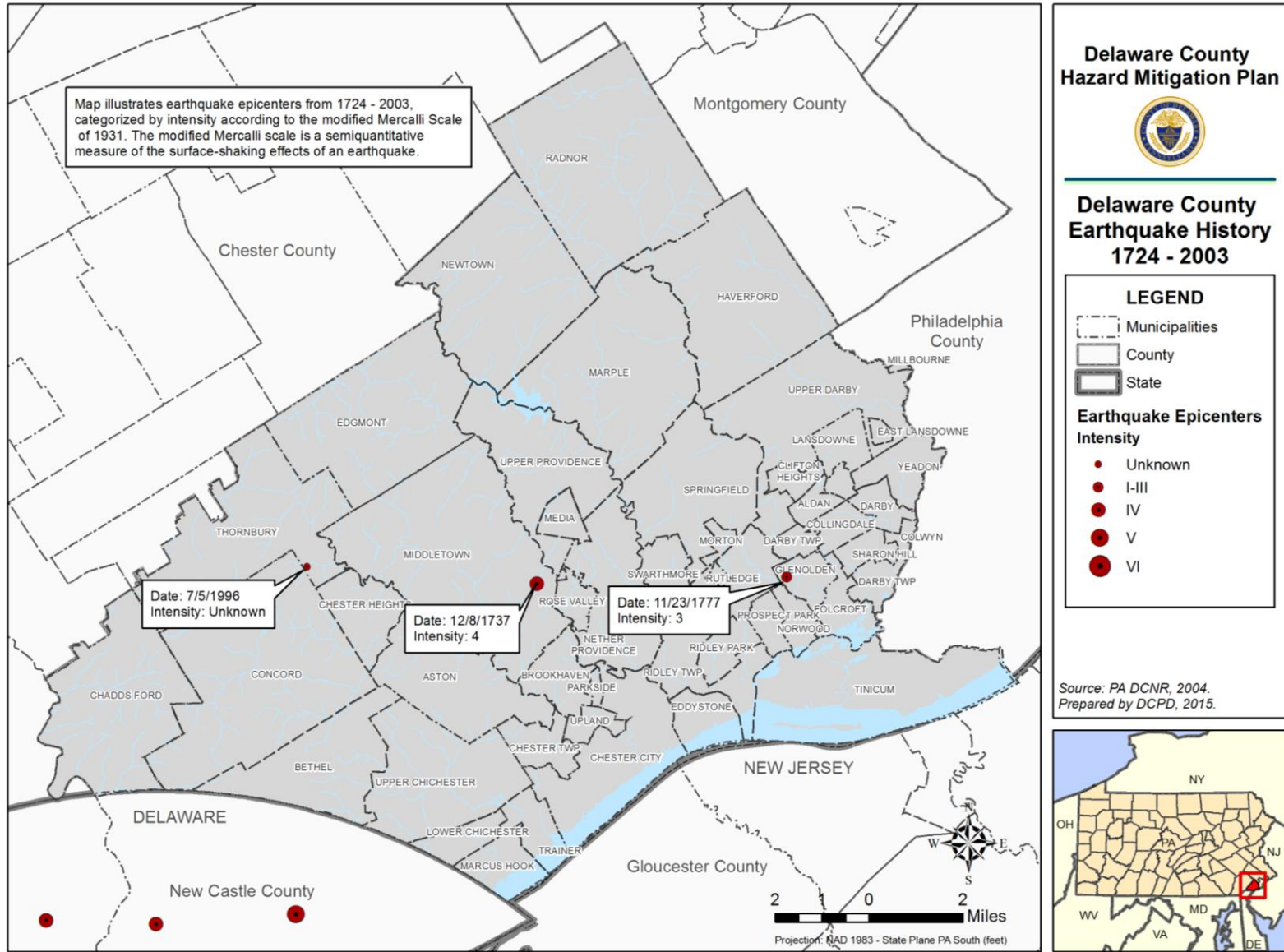
Figure 4.3.2-2: Delaware County Earthquake History.
