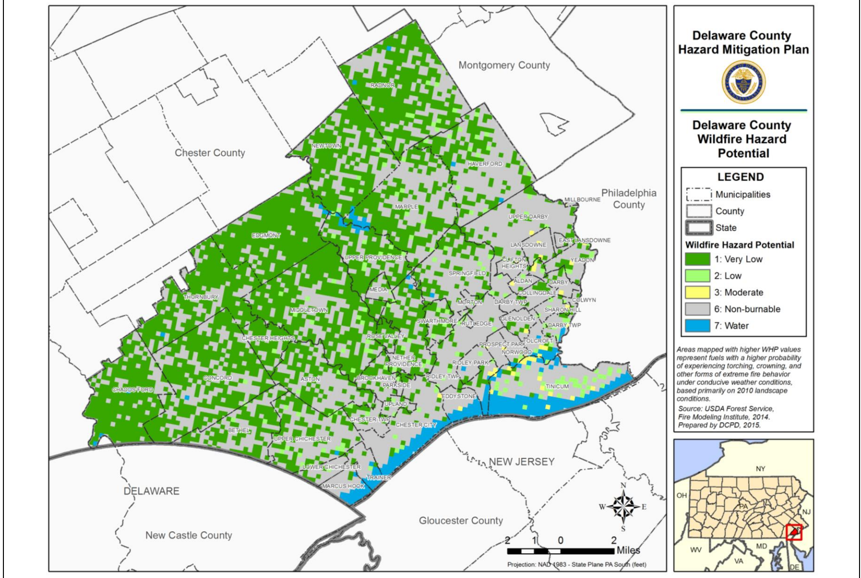
Figure 4.3.13-2: Wildfire Hazard Potential in Delaware County.
