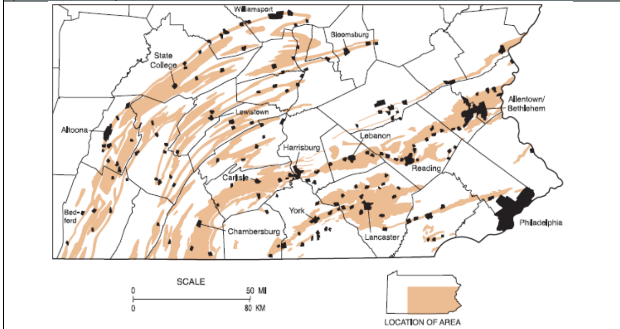
Figure 4.3.11-1: Areas in Eastern and Central Pennsylvania Susceptible to Subsidence Based on the Presence of Underlying Carbonate Rock Formations with Urban Areas Shown in Black (Kochanov, 1999).
