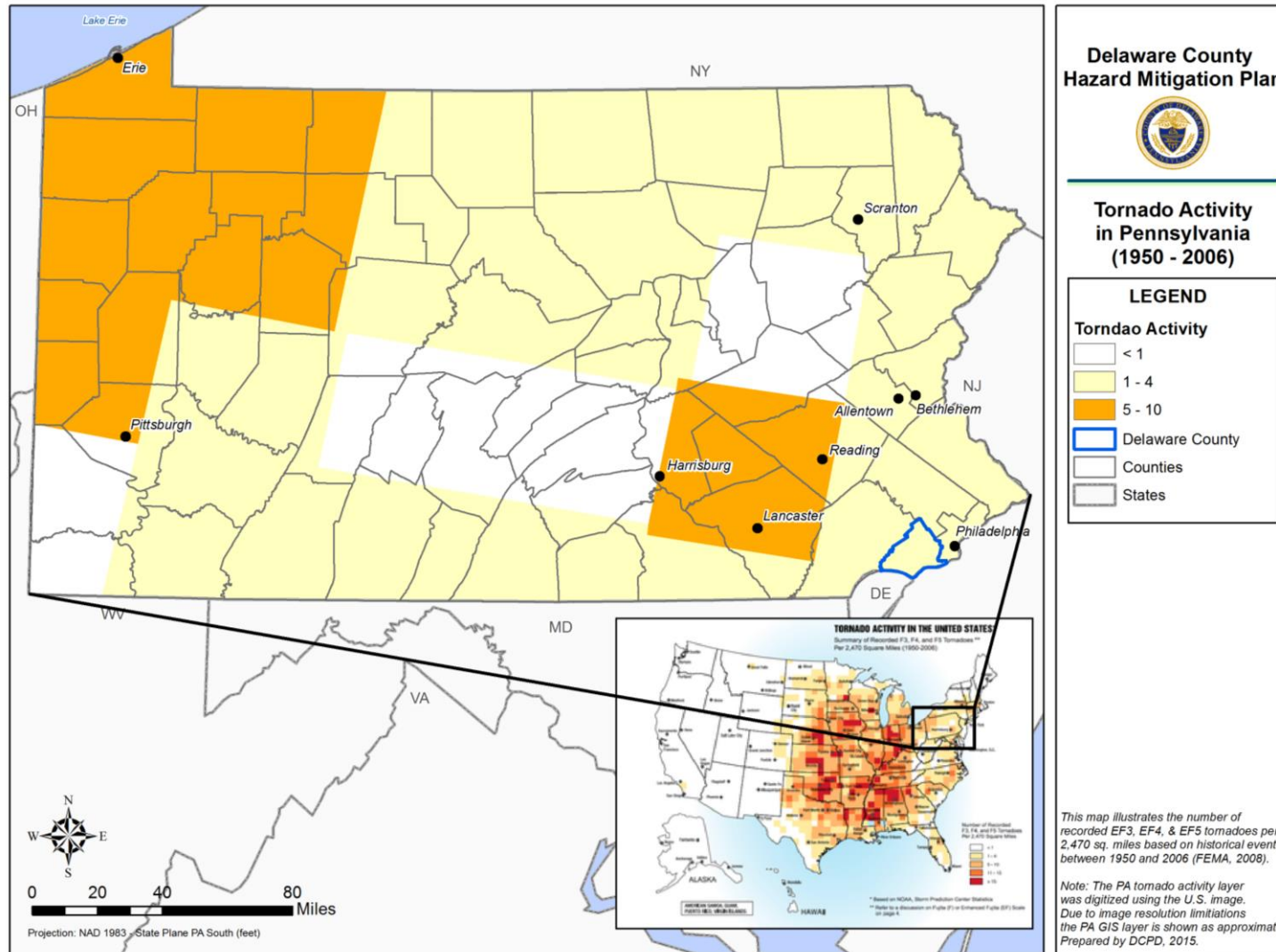
Figure 4.3.12-2: Number of Recorded F3, F4, & F5 Tornadoes per 2,470 sq. miles Based on Historical Events Between 1950 and 2006 (FEMA, 2008).
