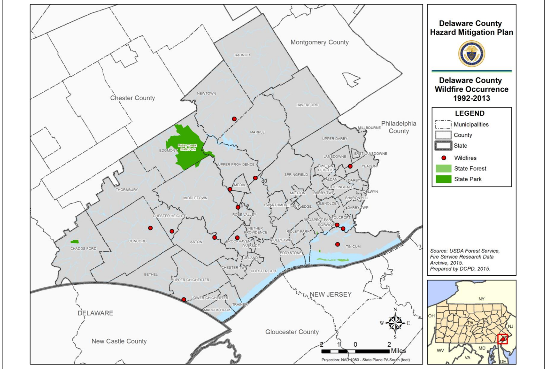
Figure 4.3.13-1: Wildfire Origins in Delaware County Between 1992 and 2013. (USDA Forest Service, 2015).
