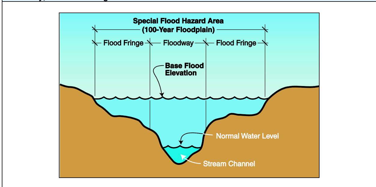
Figure 4.3.4-1: Diagram of Special Flood Hazard Area, 1% Annual Chance (100-Year) Floodplain, Floodway, and Flood Fringe.
