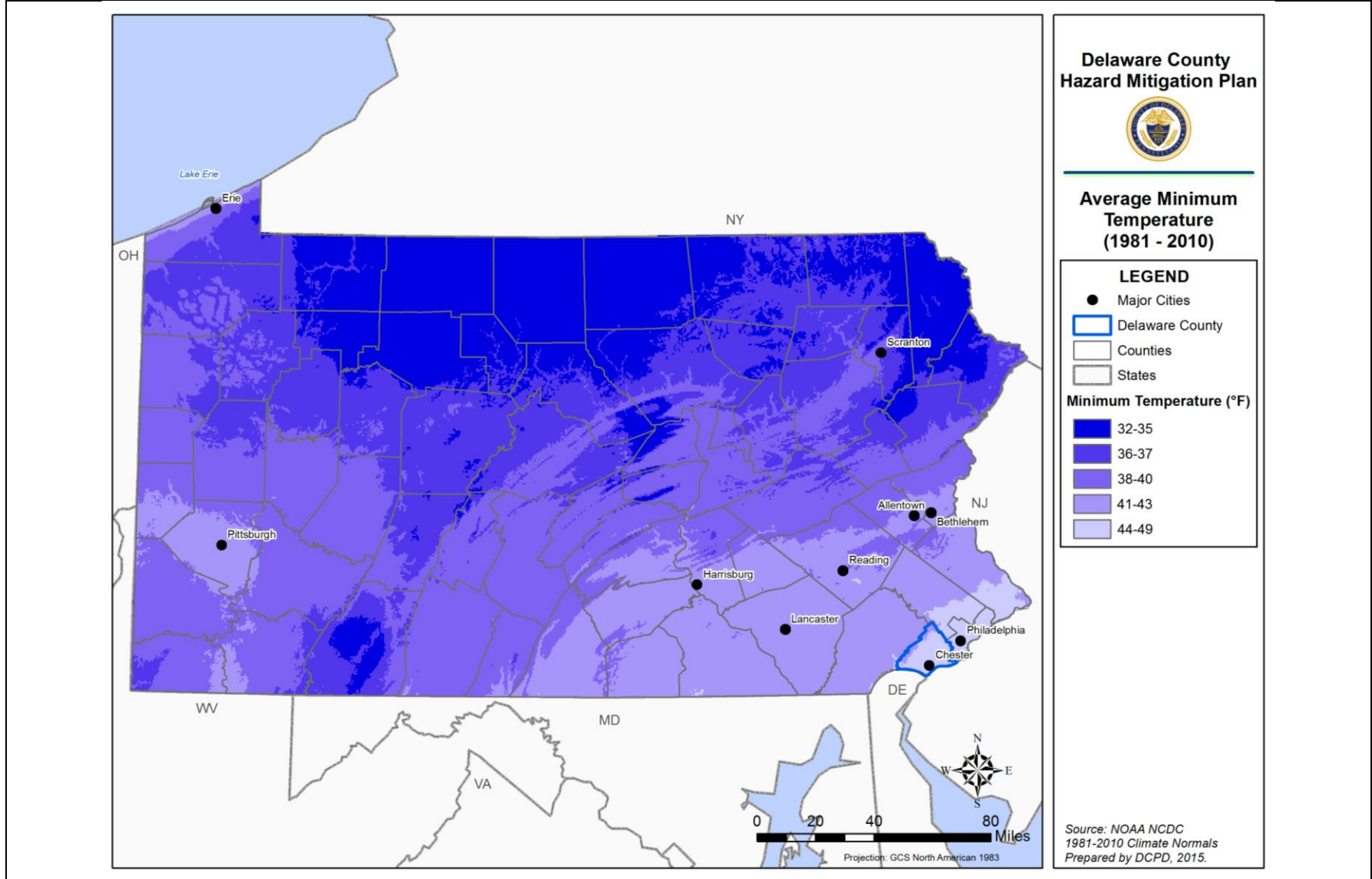
Figure 4.3.3-1: Average Minimum Temperature Based on Temperature Data Collected Between 1981 and 2010 (NOAA NCDC, 2015).
