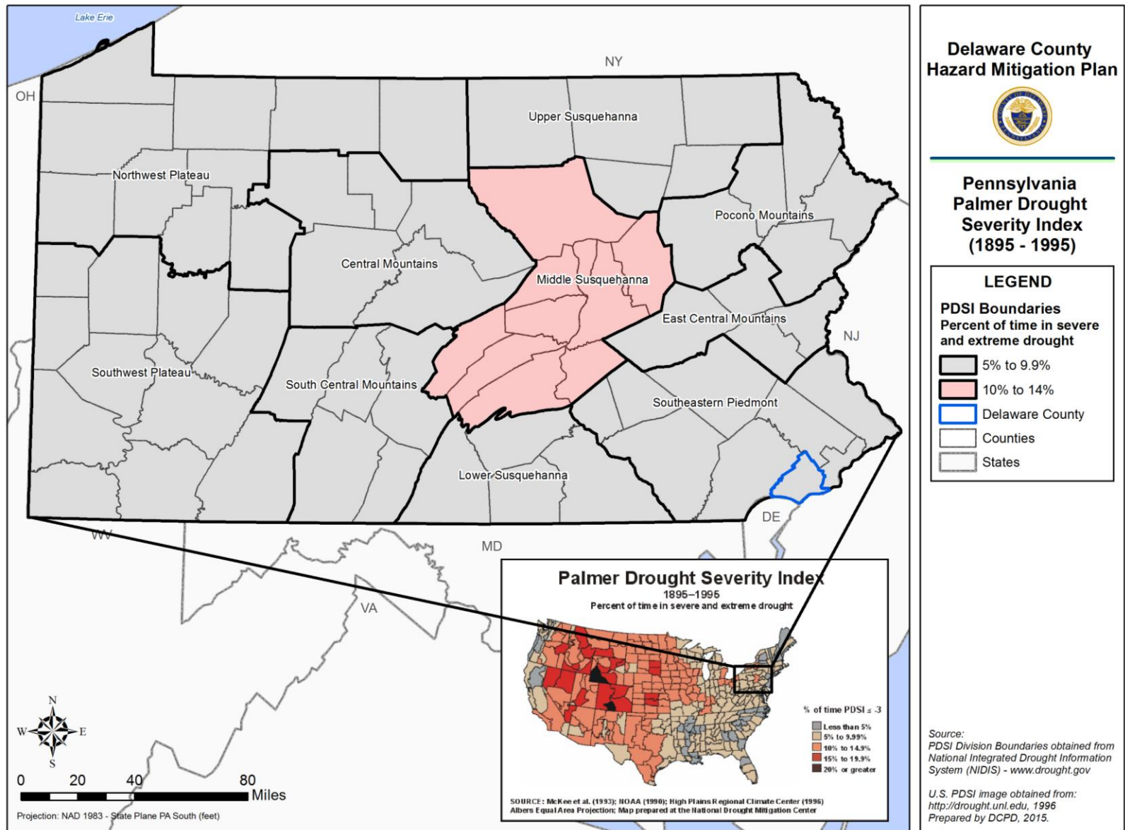
Figure 4.3.1-1: Percent of Time Areas of the United States Have PSDI values \leq -3 (NIDIS, 2010).
