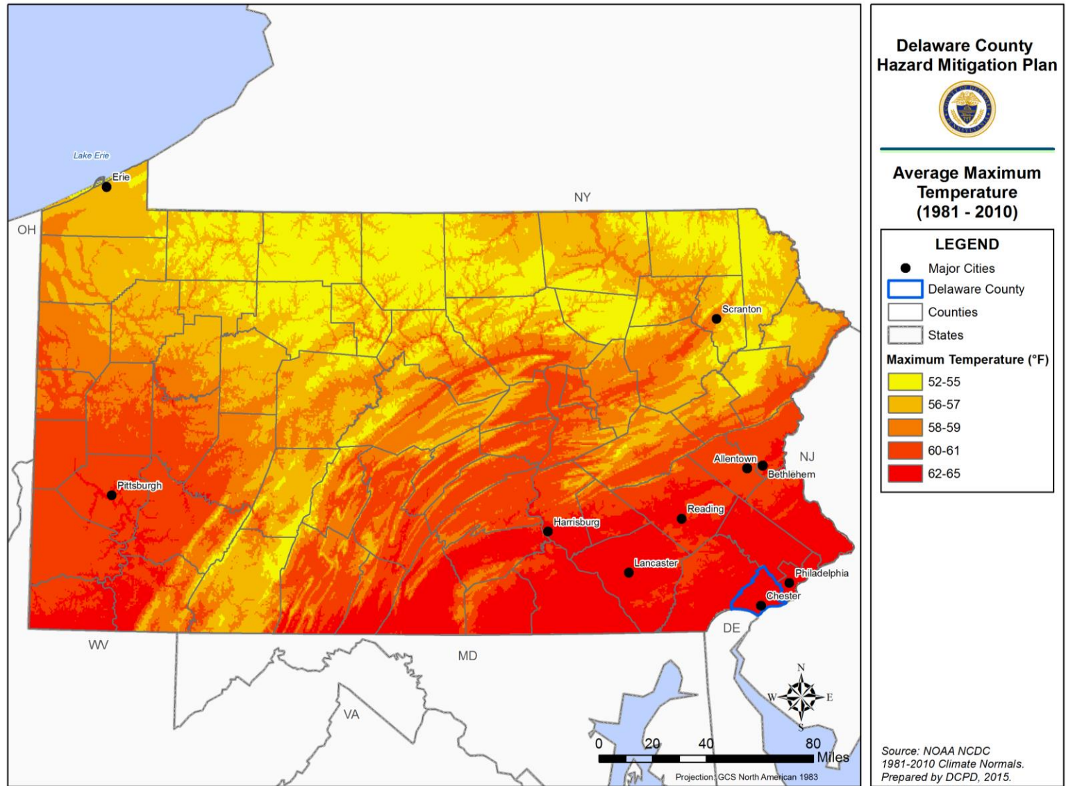
Figure 4.3.3-2: Average Maximum Temperature Based on Temperature Data Collected Between 1981 and 2010 (NOAA NCDC, 2015).
