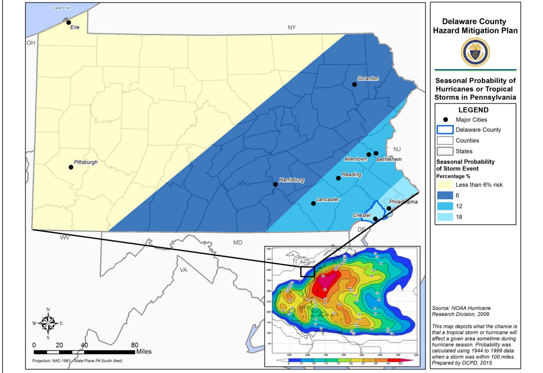
Figure 4.3.6-2: Seasonal Probability of a Hurricane or Tropical Storm Affecting Delaware County (NOAA HRD, 2009).
