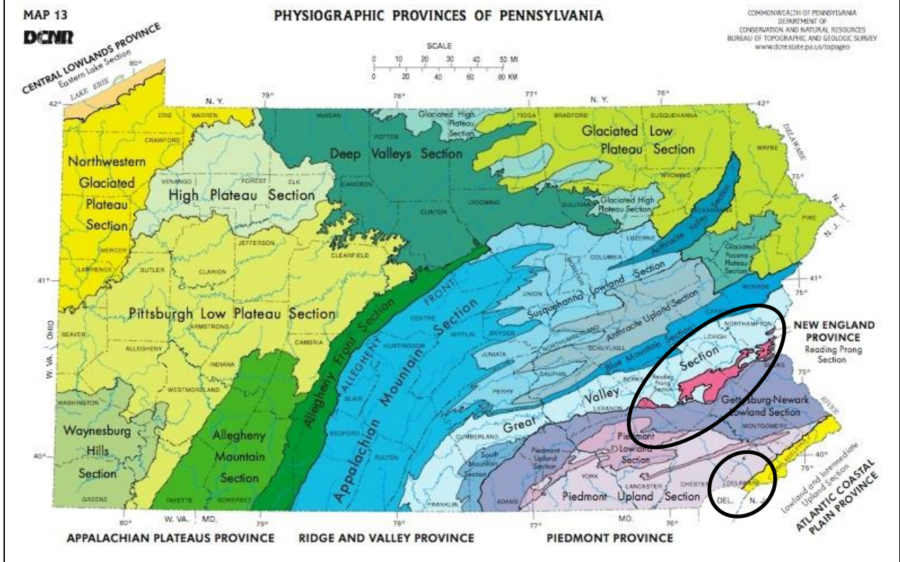
Figure 4.3.10-2: Pennsylvania Physiographic Provinces (PA DCNR, 2011).
