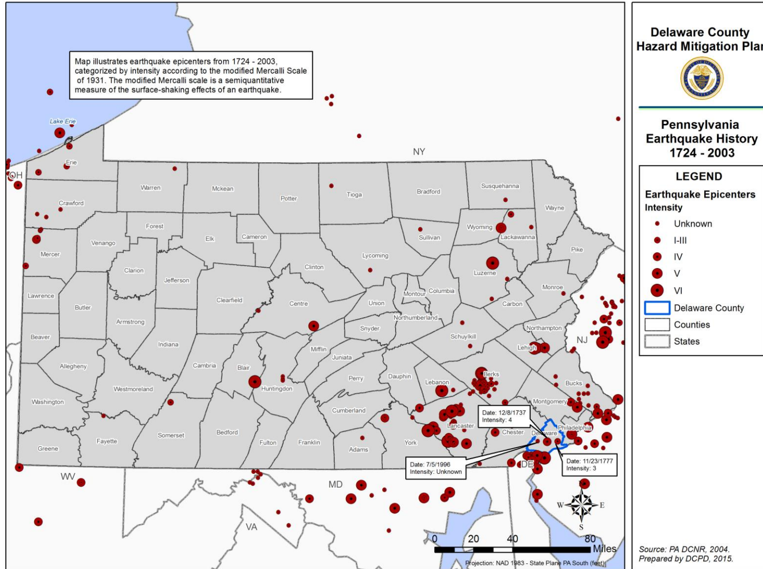
Figure 4.3.2-1: Significant Earthquake Epicenters in Pennsylvania.
