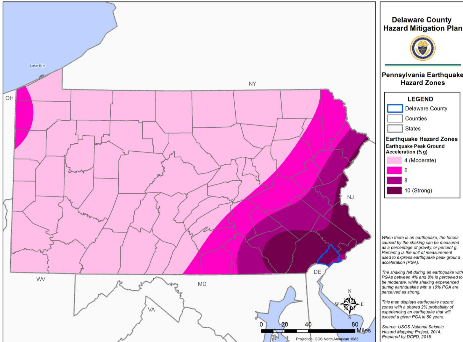
Figure 4.3.2-3: Pennsylvania Earthquake Hazard Zones (USGS National Seismic Mapping Project, 2014).
