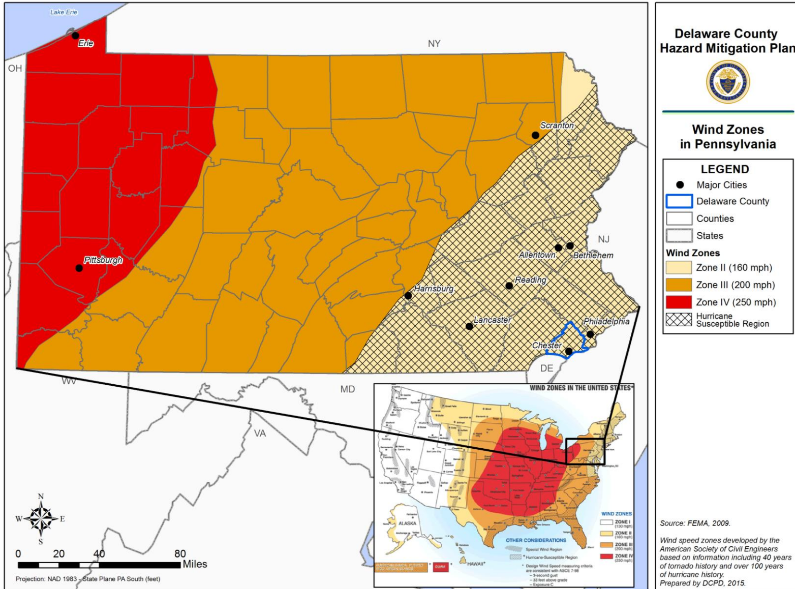
Figure 4.3.6-1: Wind Zones in Pennsylvania and Delaware County (FEMA, 2009).
