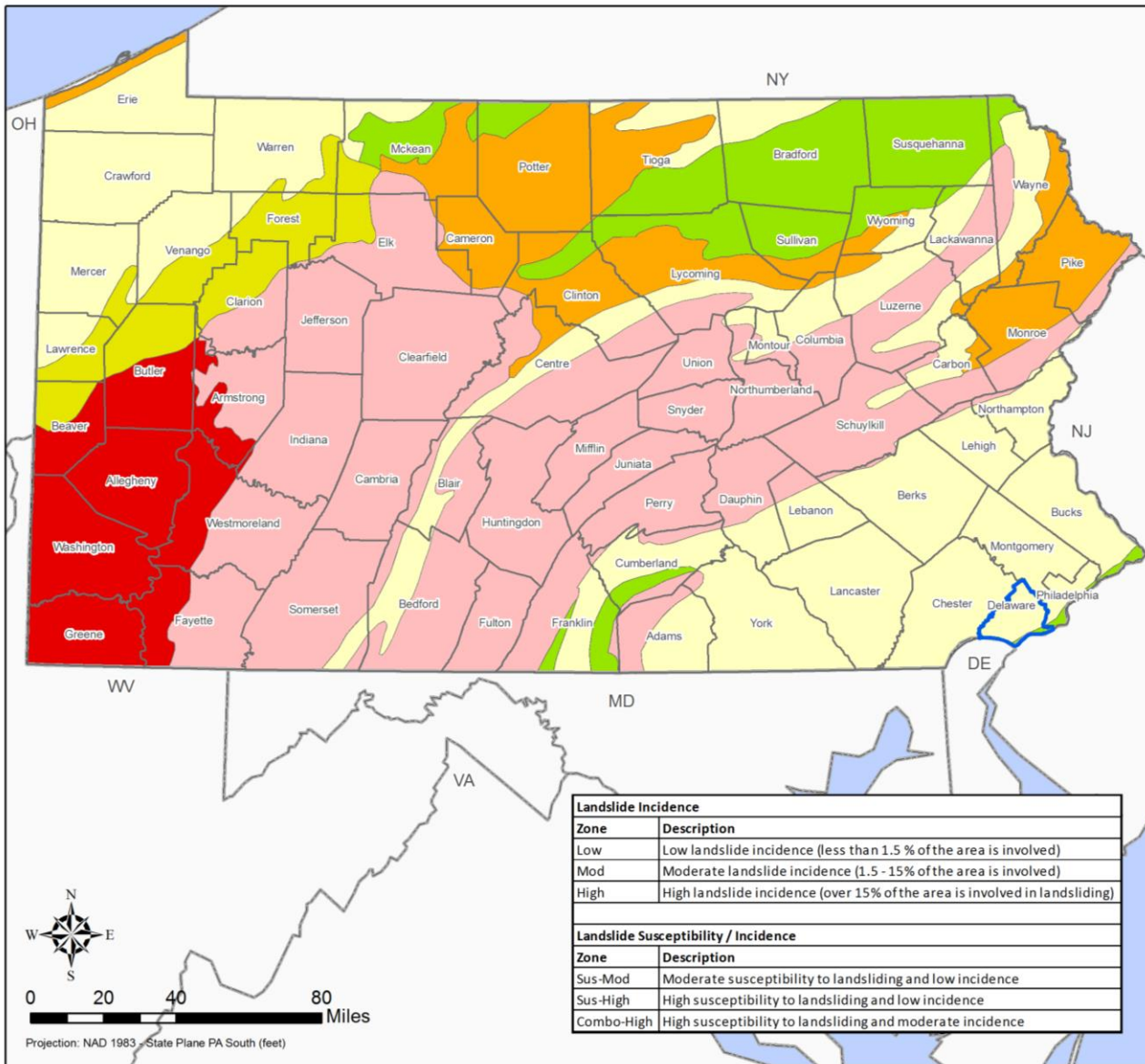
Figure 4.3.7-1: General Landslide Hazard Areas in Delaware County (USGS, 2001).
