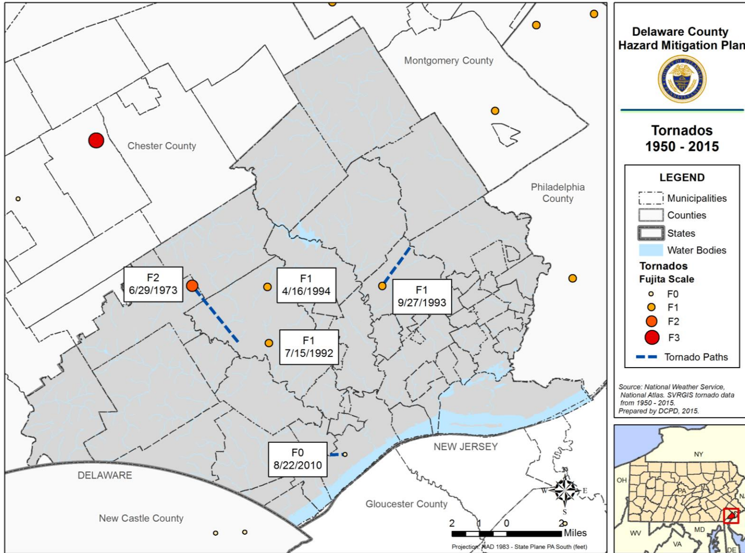
Figure 4.3.12-1: Tornadoes That Have Touched Down in Delaware County Between 1950 and 2015 (NWS via National Atlas, 1950-2015).
